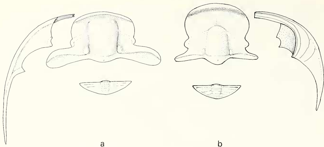
TEXT-FIG. 25. Comparative reconstructions of a primitive trinucleacean ( a ) and the late Middle Cambrian Liostracinidae ( b ), to show similarity apart from retained primitive characters of the latter. a , Orometopus (Tremadoc; new reconstruction), fused cheeks are indicated by 'broken' doublure. b , Liostracina , cranidium and cheek of L. nolens (after Öpik 1967, pl. 35, figs. 1 and 4), with undoubted median suture, and pygidium of same genus (after Chu 1959, pl. 1, fig. 31). Both \times 8 approx.
